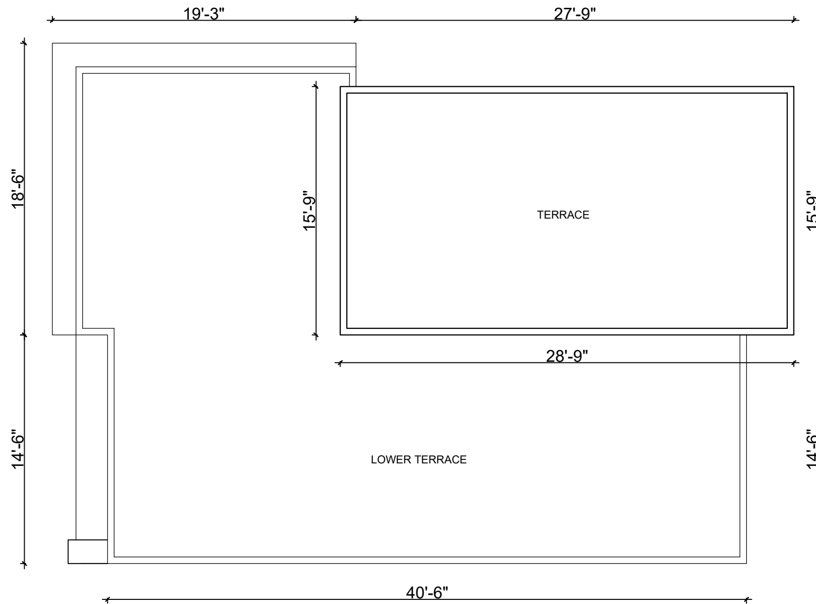
ROOF PLAN
