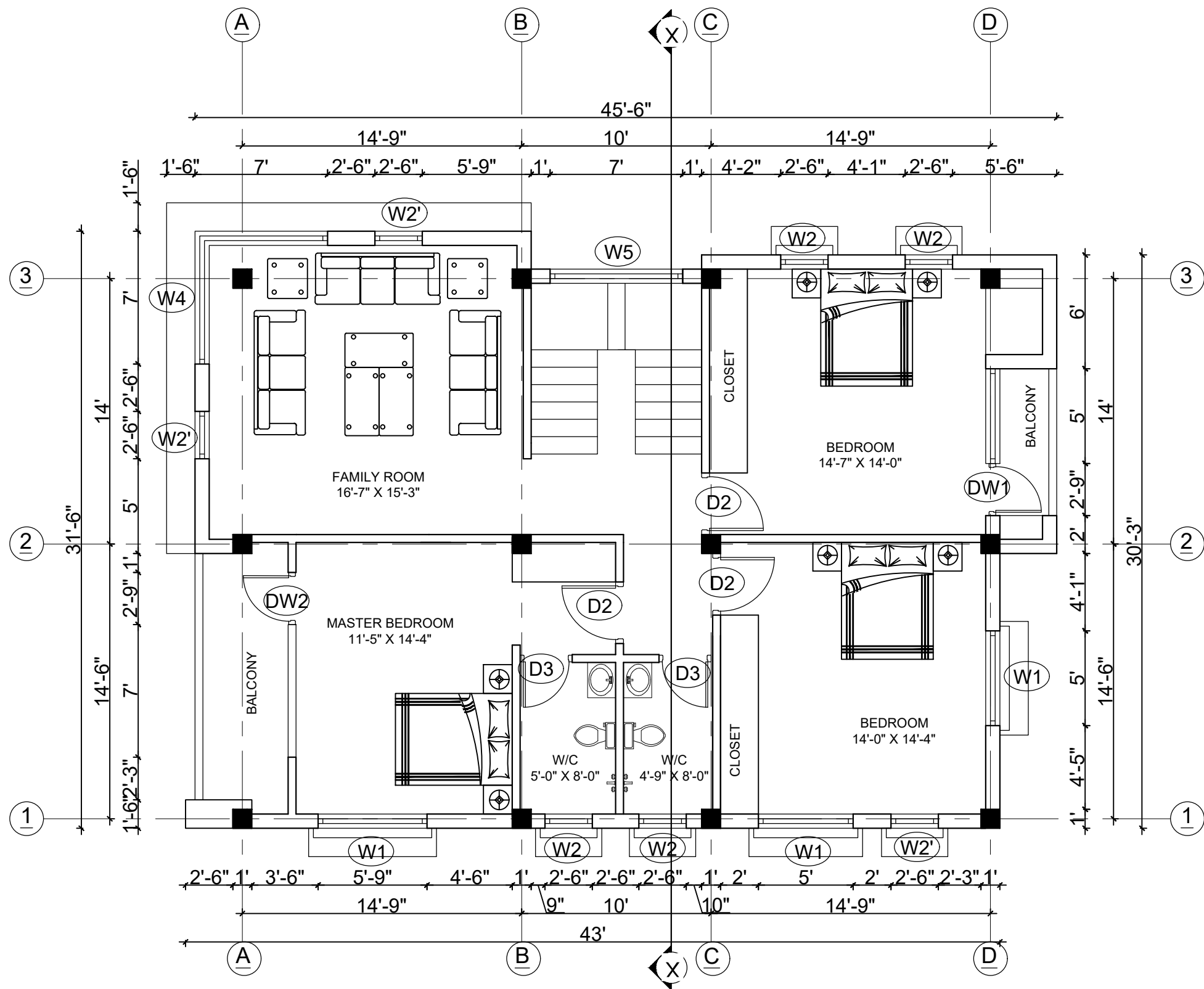
FIRST FLOOR PLAN FLOOR AREA: 1319.31 SQ.FT
