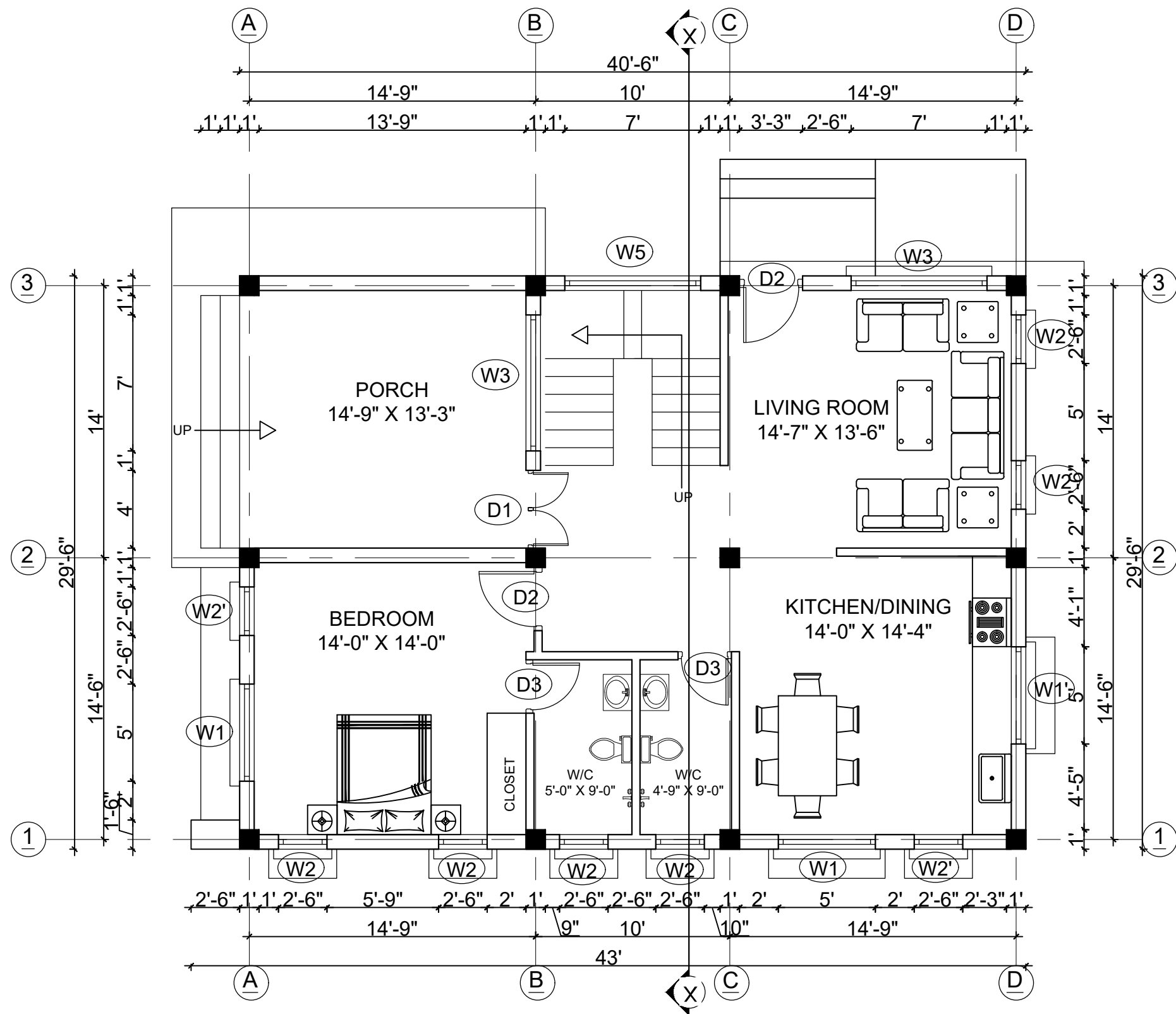
GROUND FLOOR PLAN FLOOR AREA: 1194.75 SQ.FT
