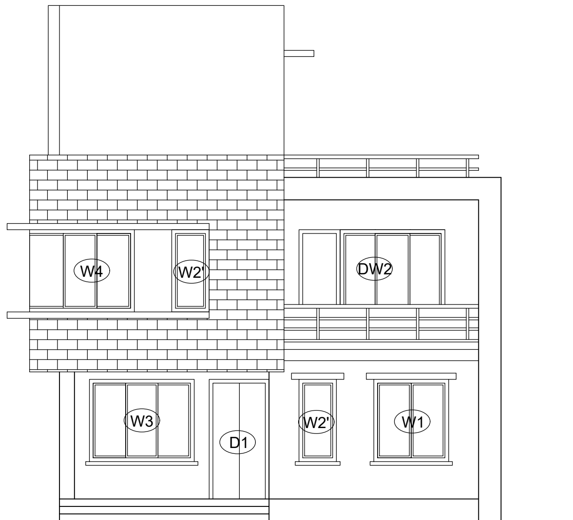
WEST ELEVATION
