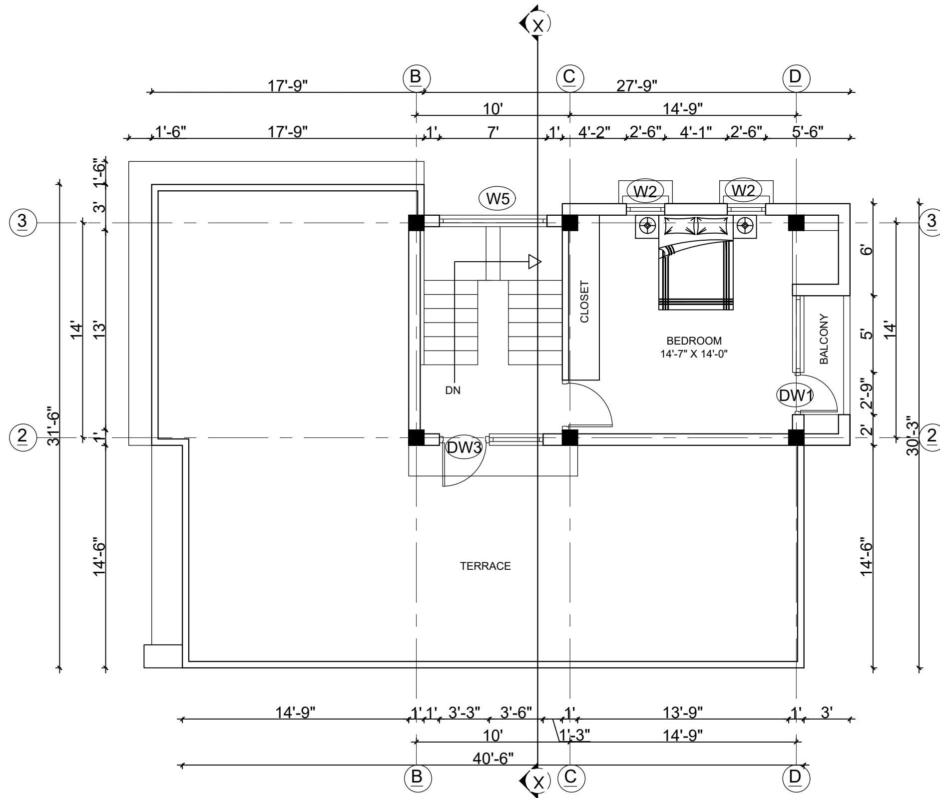
SECOND FLOOR PLAN FLOOR AREA: 445.31 SQ.FT
